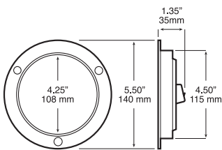
Flange mount
