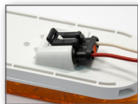
Rear of light showing built-in AMP compatible receptacle & plug
