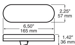
PM-1220A-10 light module
