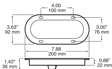
Flange mount
