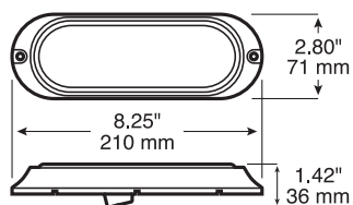
Surface mount with bracket
