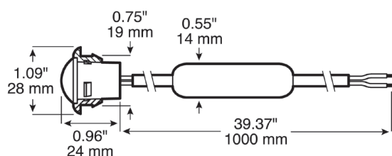
Dimensions shown with rubber grommet installed
