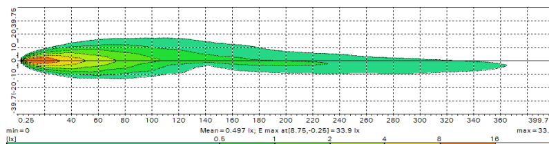
Illuminance on road surface: high beam
