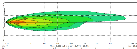
Illuminance on road surface: low beam (LHT beam pattern shown)
