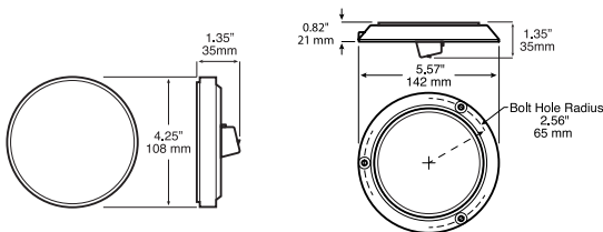
PM-872W light module
