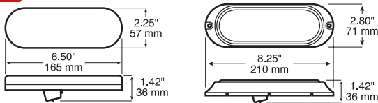
PM-870W light module
